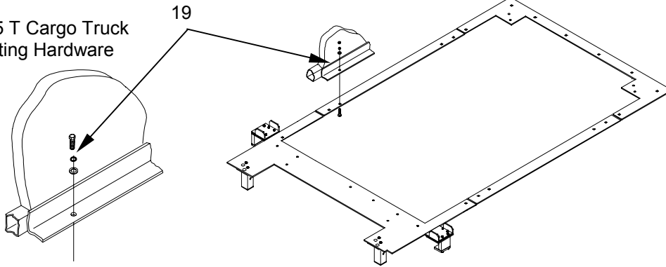
M1083, 5 T MTV or M1095, 5 T MTV Trailer Mounting Hardware
